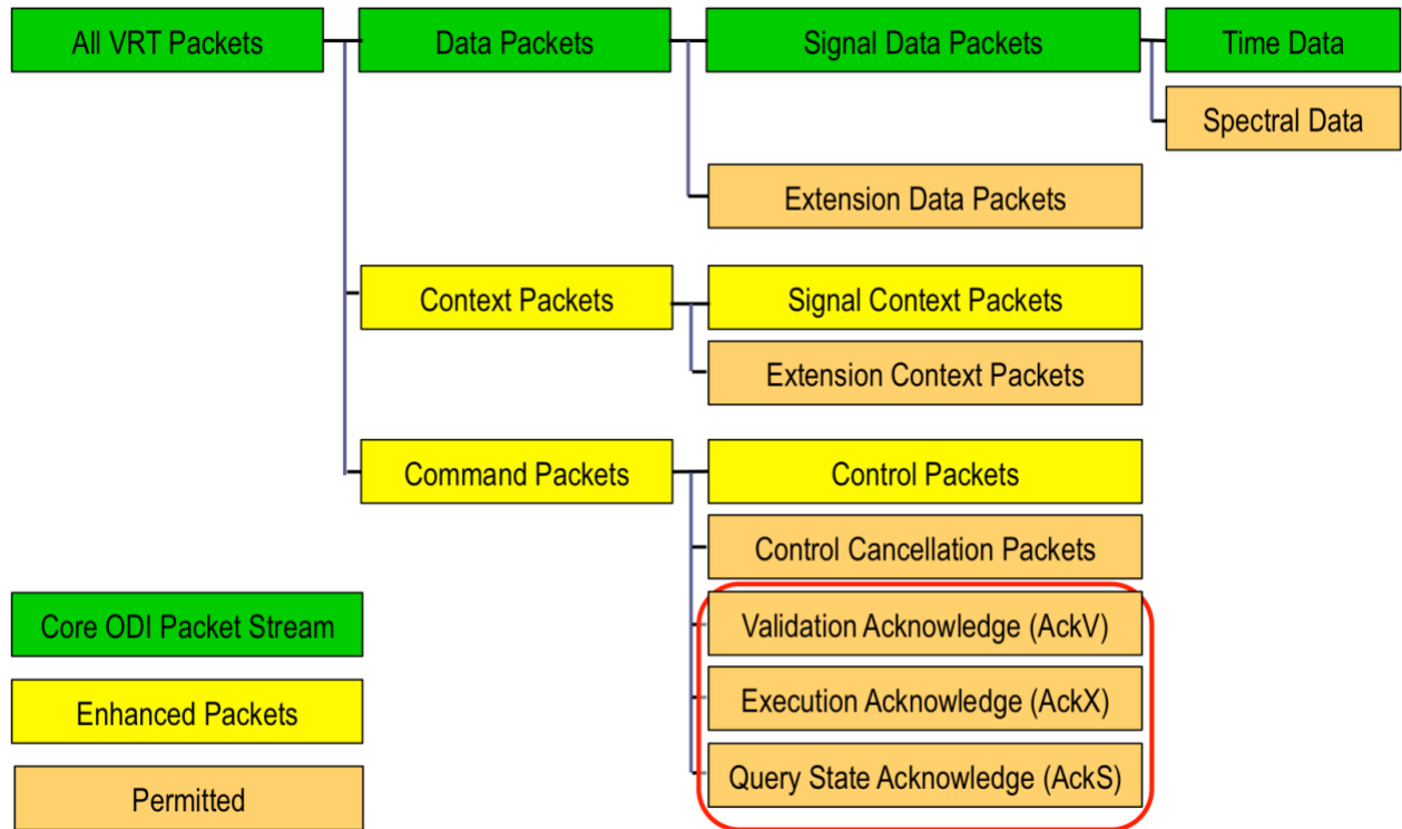
Figure 3-31: VRT Control Acknowledge Packets
