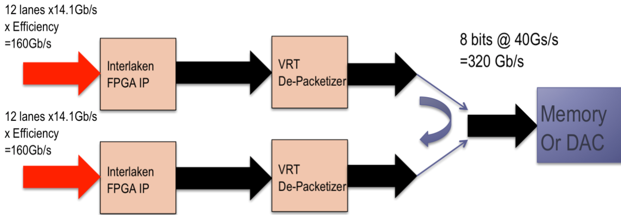
Figure 4-3: Single-channel port aggregation example – Reception
