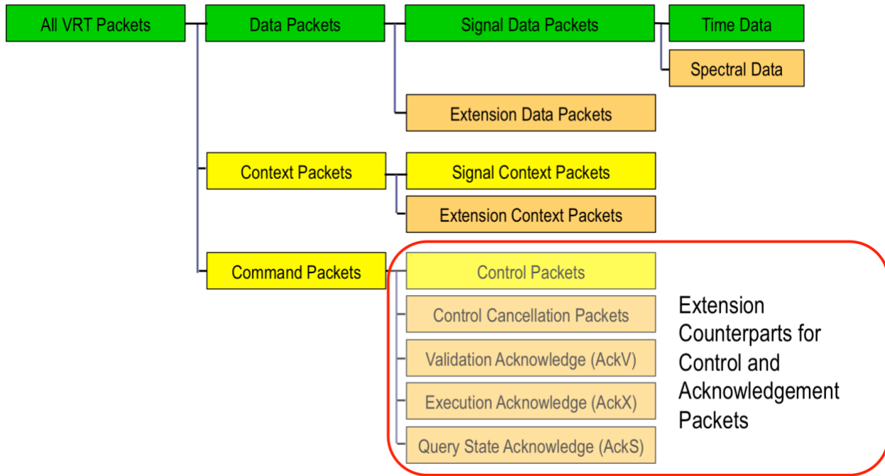
Figure 3-32: VRT Extension Command Packets
